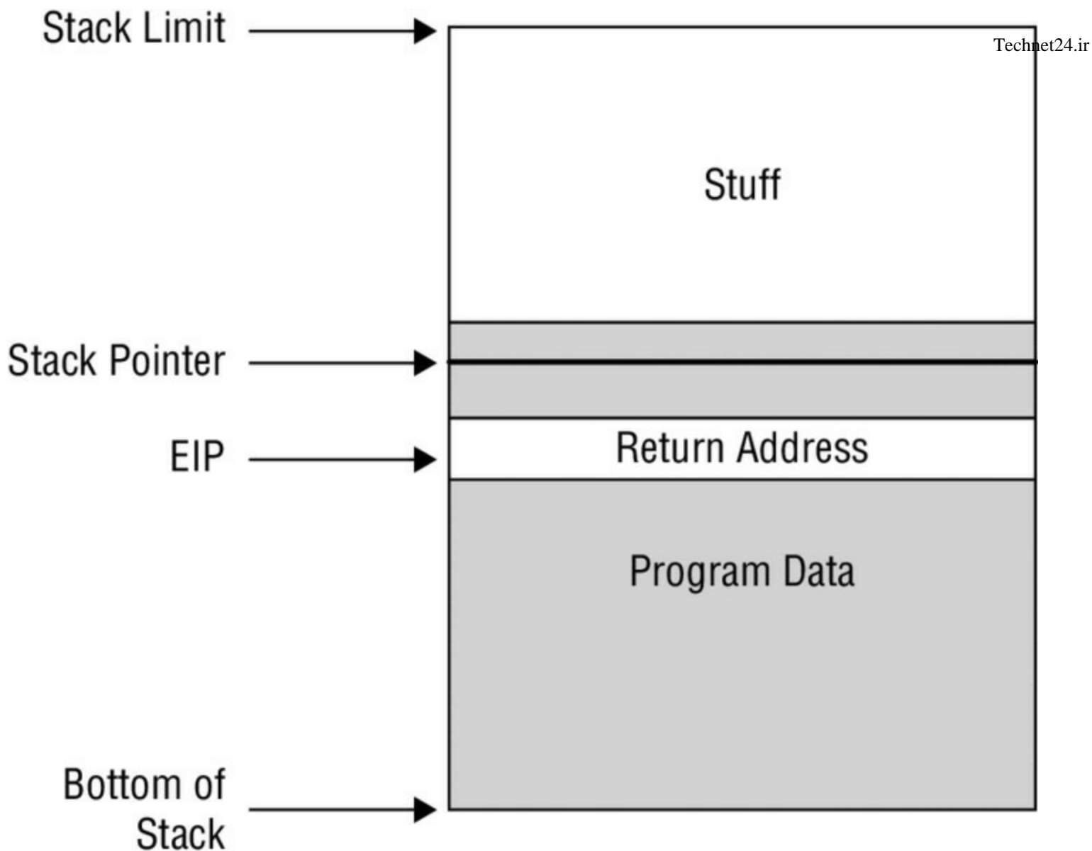
Figure 11.1 Basic program stack
