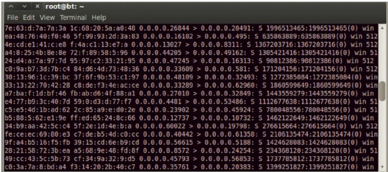
Figure 9.2 Macof MAC flood
