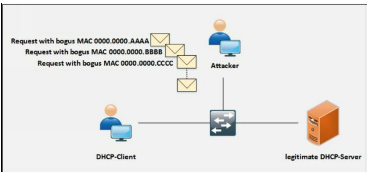
Figure 8-08 DHCP Starvation Attack
