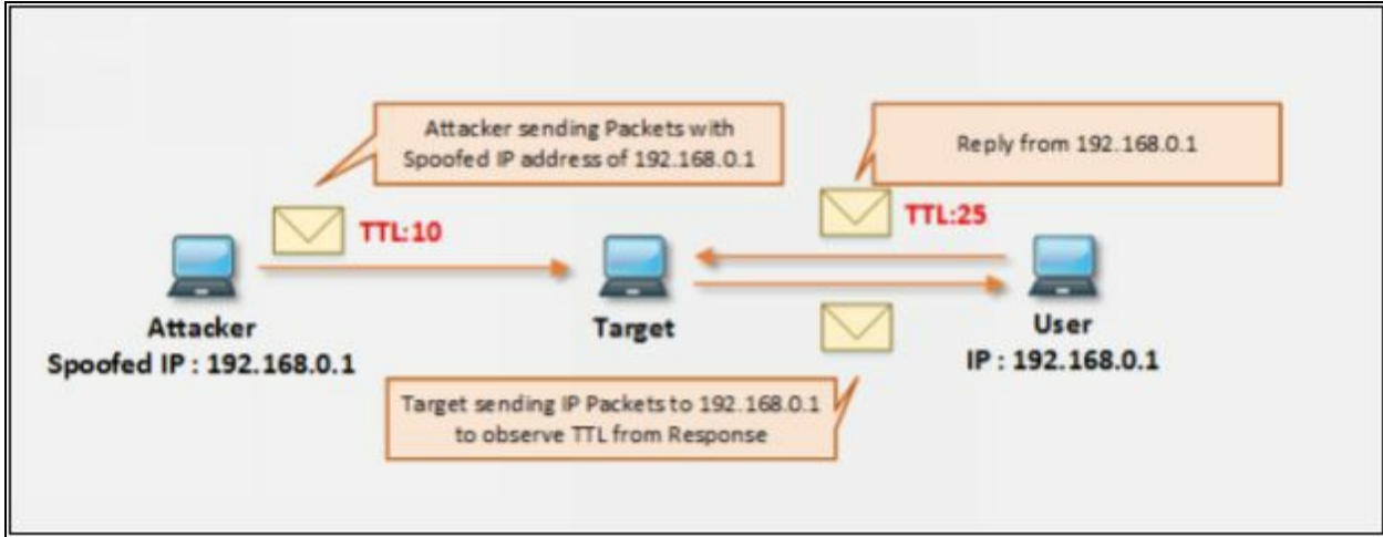
Figure 3-51 Direct TTL Probing
