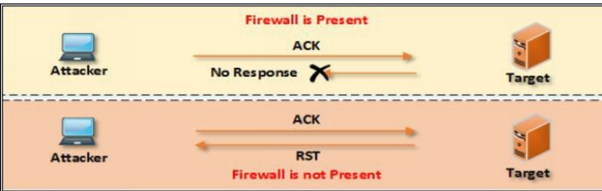
Figure 3-29 Ack Flag Probe Scanning Response
