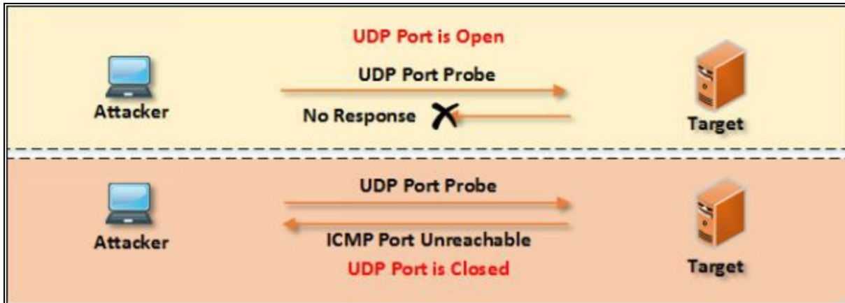
Figure 3-34 UDP Scanning Response
