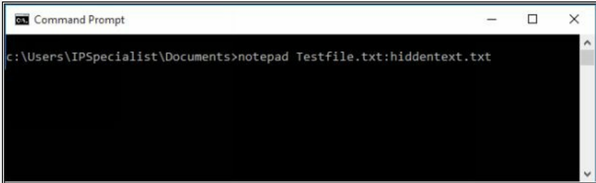
Figure 6-41 Creating Hidden File
