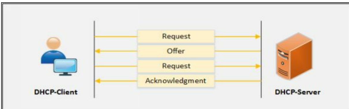
Figure 8-06 IPv4 DHCP process
