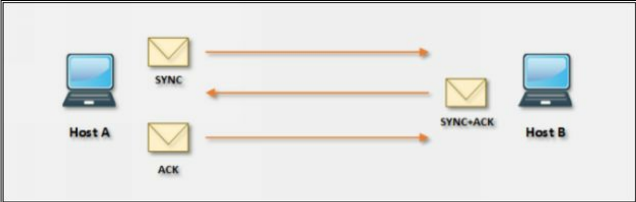
Figure 3-03 TCP Connection Handshaking
