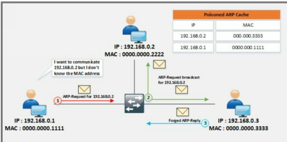
Figure 8-11 ARP Spoofing Attack
