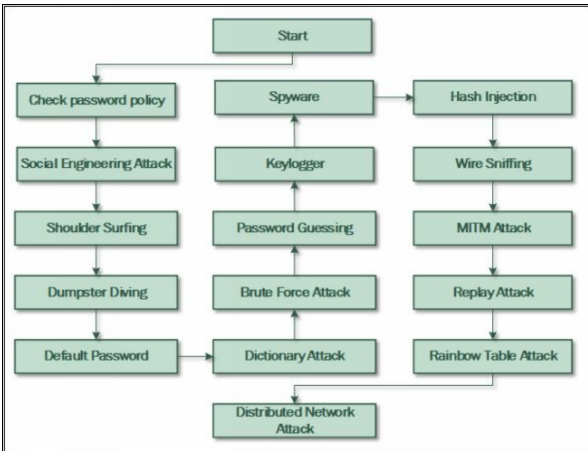
Figure 6-11 Password Cracking Flow Chart
