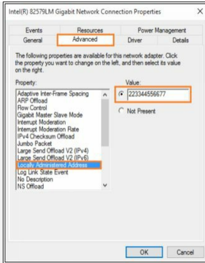
Figure 8-19 Network Adapter Properties
