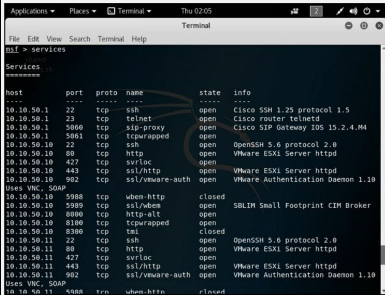
Figure 2-82: Service Scan results
