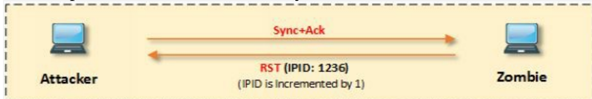
Figure 3-33 Step#03 Idle Scanning
