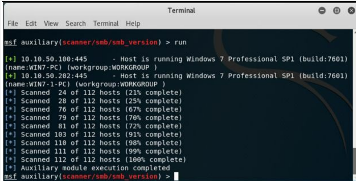
Figure 2-84: Running SMB Scan
