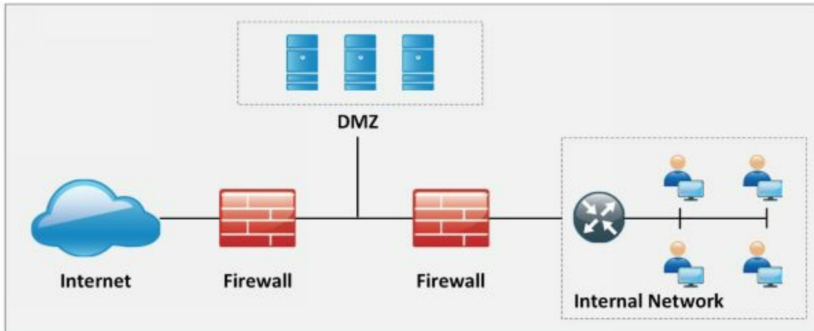
Figure 12-06. Multi-Homed Firewall
