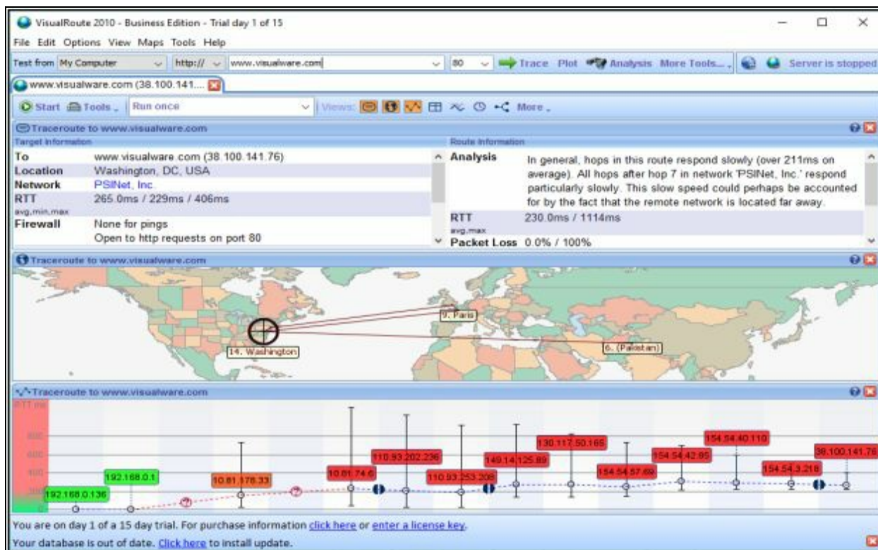
Figure 2-43 Visual Route Application
