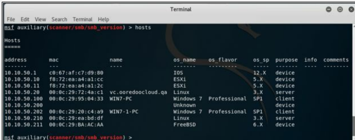
Figure 2-85: SMB Scan results
