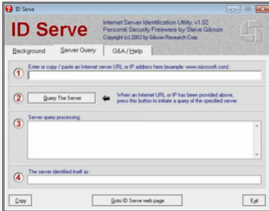
Figure 13-04 ID Serve Application
