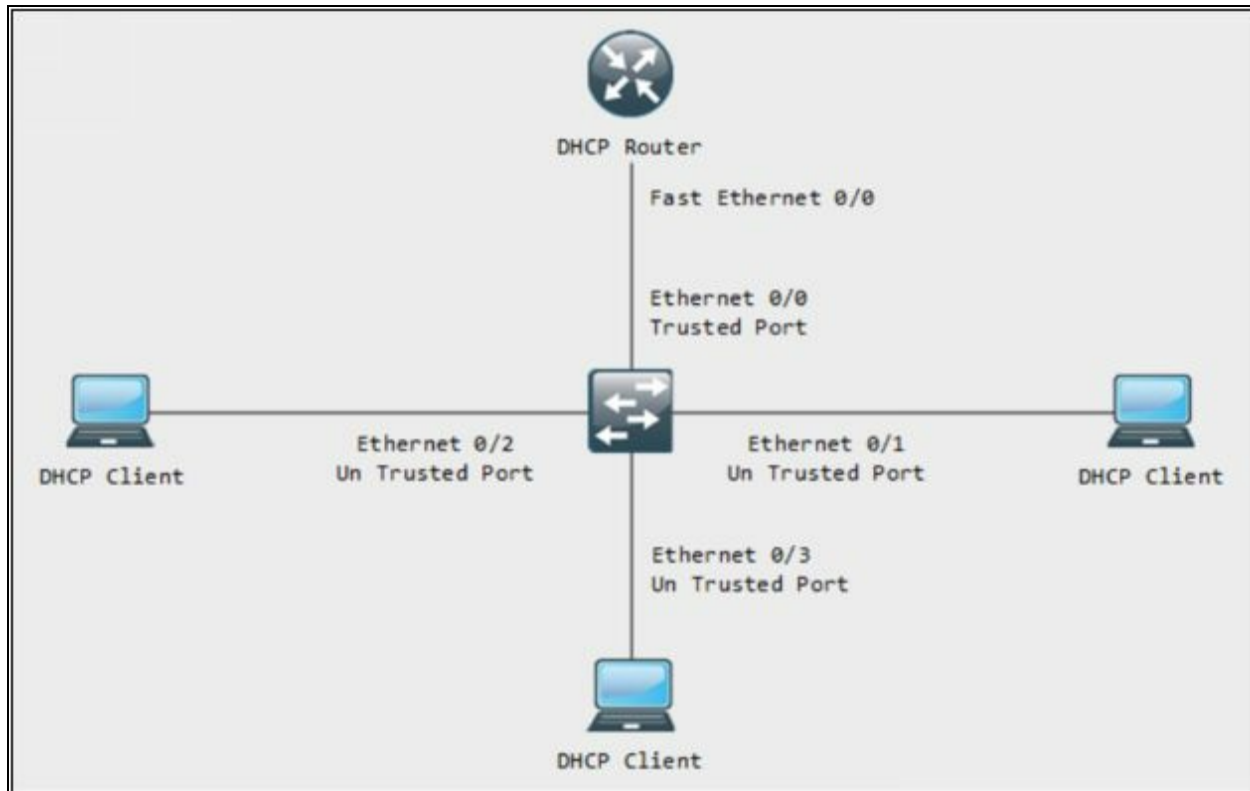
Figure 8-12 Configuring DHCP Snooping
