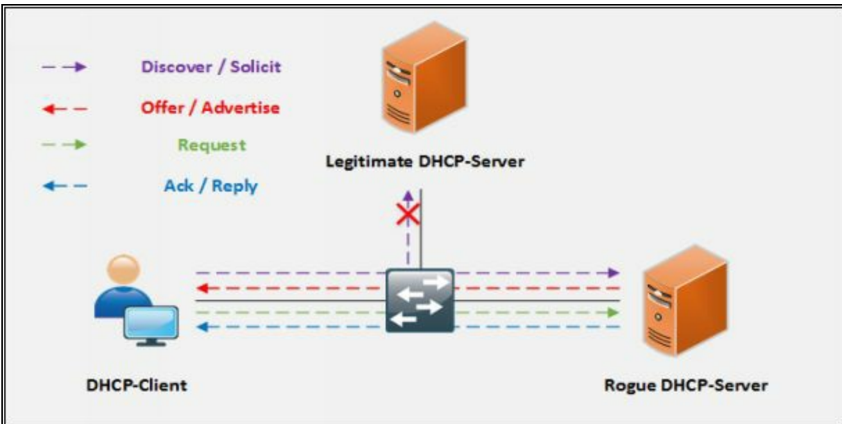
Figure 8-09 Rogue DHCP Server Attack
