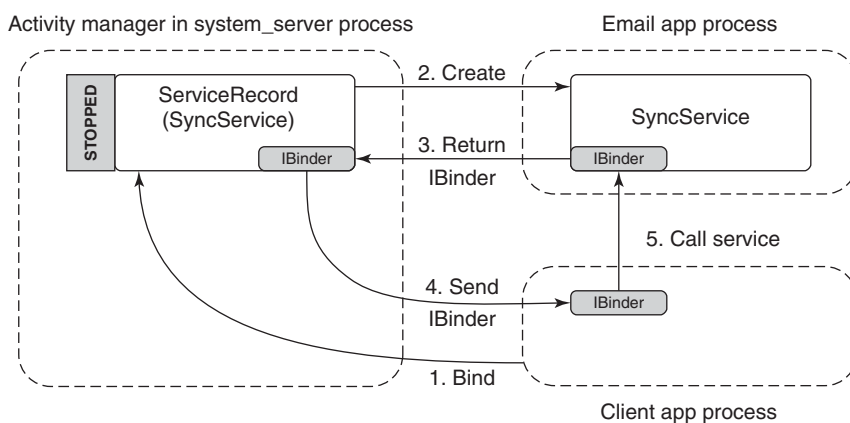
Figure 10-59. Binding to an application service.
