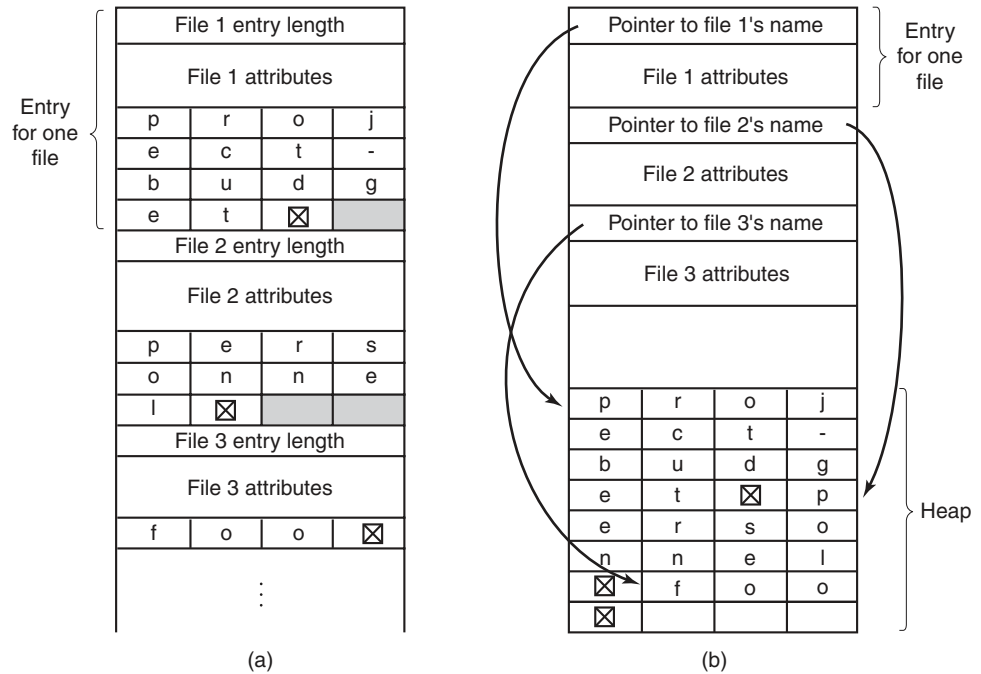
Figure 4-15. Two ways of handling long file names in a directory. (a) In-line. (b) In a heap.
