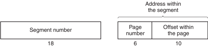
Figure 3-35. A 34-bit MULTICS virtual address.
