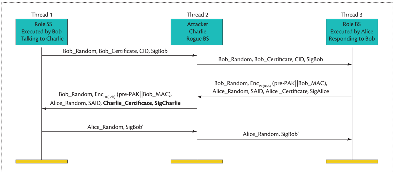
Figure 1. Man-in-the-middle attack on PKMv2-RSA. Subscriber station (SS) Bob is talking to attacker Charlie. Base station (BS) Alice thinks Bob is talking to her.
